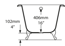
Rim Detail
